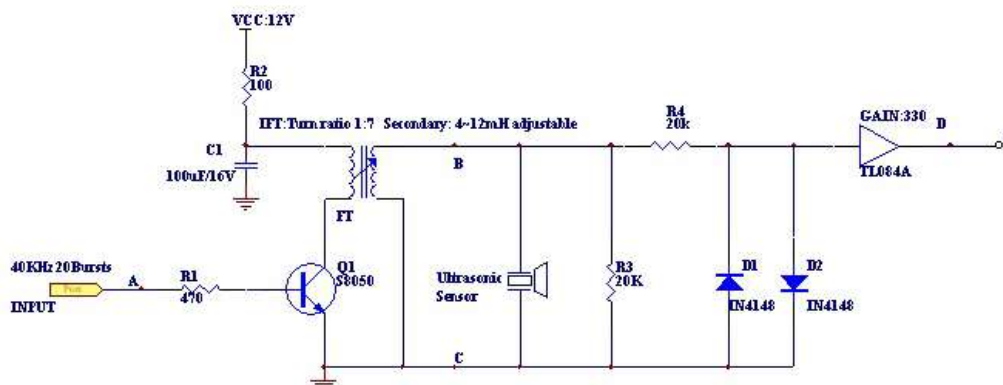
FIG4 SIMULATION TEST CIRCUIT
